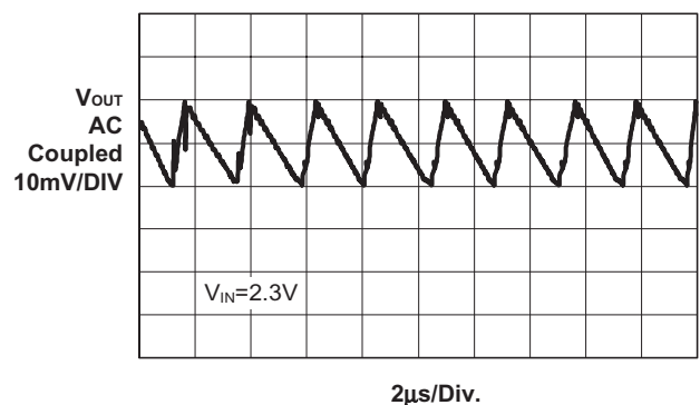
Output Ripple for 100mA Load AAT3110-3.3
